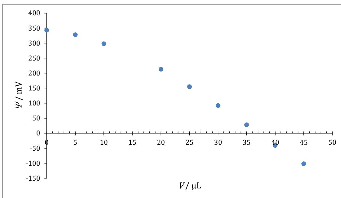
Slika 17. Ovisnost potencijala strujanja suspenzije \text{CeO}_2 ( \gamma(\text{CeO}_2) = 0,1 \text{ g dm}^{-3} ) u HCl ( c = 0,001 \text{ mol dm}^{-3} ) i NaCl ( c = 0,01 \text{ mol dm}^{-3} ) o volumenu dodanog polielektrolita ( c(\text{NaPSS}) = 4,83 \times 10^{-5} \text{ mol dm}^{-3} ), \theta = 25^\circ\text{C}
