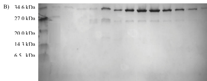
Figure 27. A) Gel filtration chromatogram of Ni-NTA agarose eluate containing His 6 -tagged Sec13 (AA12 I→F ) copurified with Sec31 372-411 B) SDS PAGE of fractions A2-A4, B4-B13. Lane 1 is the protein marker
