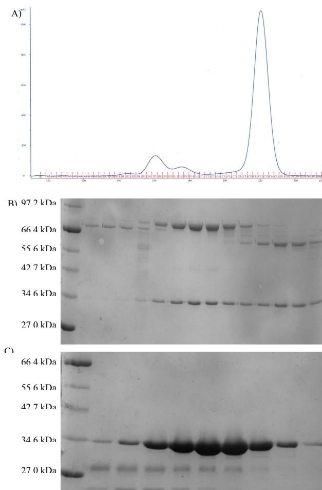
Figure 21. A) Gel filtration chromatogram of Ni-NTA agarose eluate containing His 6 -tagged Sec13 (AA12 L-F ) copurified with Nup145C B) SDS PAGE of fractions B1-B14 C) SDS PAGE of fractions C8-D1; Lane 1 is the protein marker in both B and C
