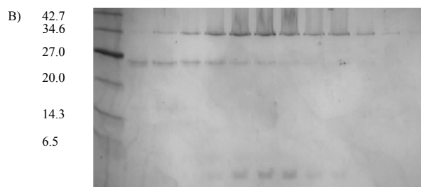
Figure 26. A) Gel filtration chromatogram of Ni-NTA agarose eluate containing His 6 -tagged wild type Sec13 copurified with Sec31 372-411 B) SDS PAGE of fractions B2-B13. Lane 1 is the protein marker
