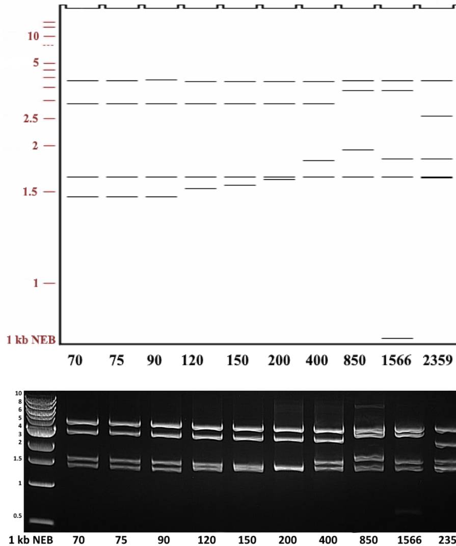
Figure 9. PvuII-digested pBsd-(70-2359) after the recombineering experiment.
