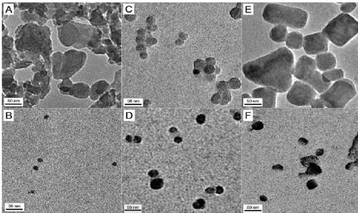
Slika 6. TEM snimke agregiraju ih estica nC_{60} : a) velike aq/ C_{60} b) male aq/ C_{60} c) velike son/ C_{60} d) male son/ C_{60} e) velike THF/ nC_{60} f) male THF/ nC_{60} (izvor: Lyon Y.D., Adams K.L., Falkner C.J., Alvarez J.J.P. (2006): Antibacterial Activity of fullerene Water Suspensions: Effects of Preparation Method and Particle Size. Environmental Science & Technology , 40, 4360-4366)
