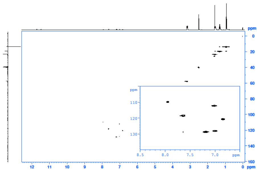
Slika P74. HSQC spektar spoja 5H_2 s TBAOAc u DMSO-d_6 ( n(TBAOAc) / n(5H_2) \approx 15 ) (400 MHz).
