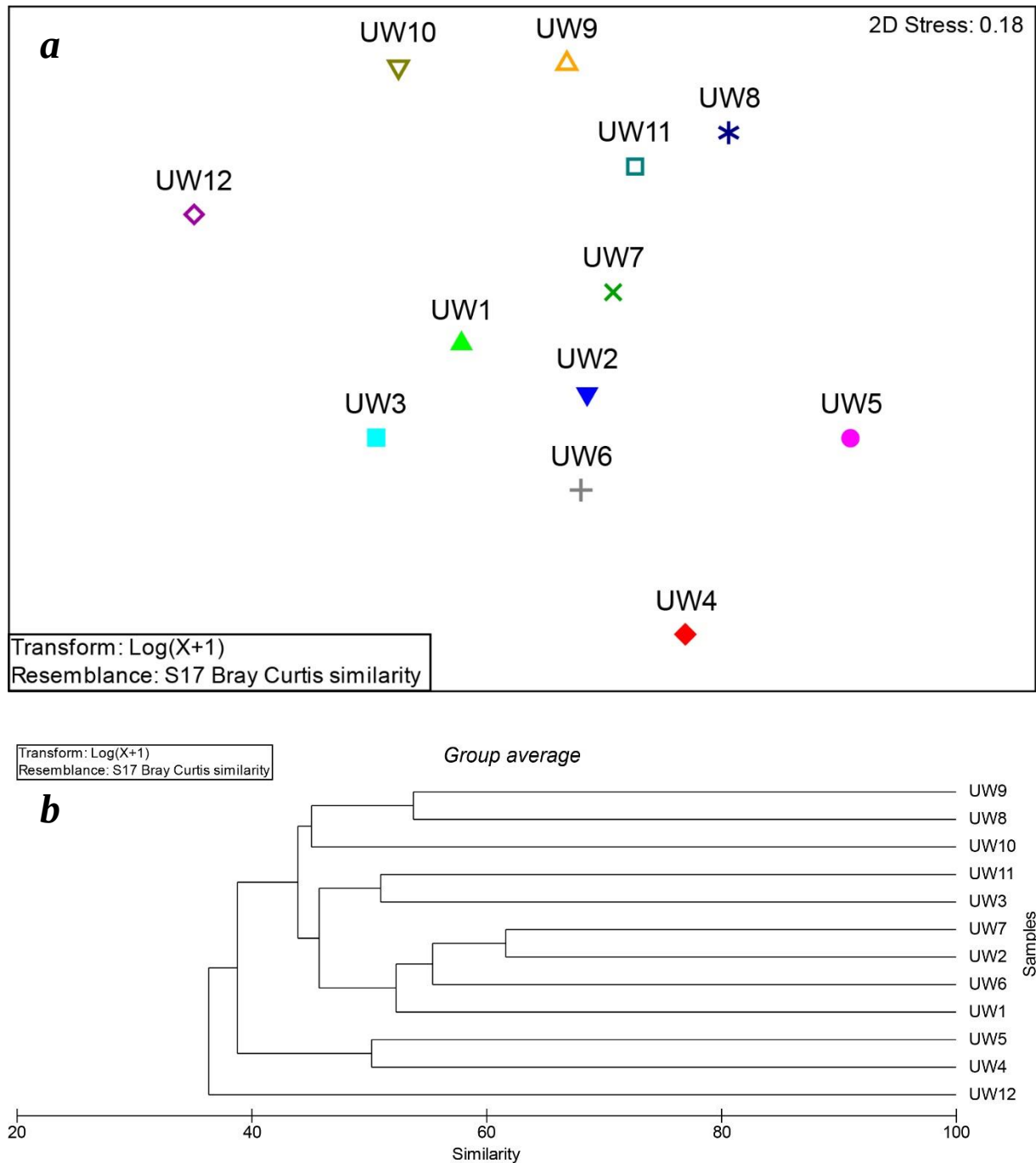
Fig. 29. Multivariant analyses of underway samples of phytoplankton: a) nMDS; b) hierarchical clustering.
