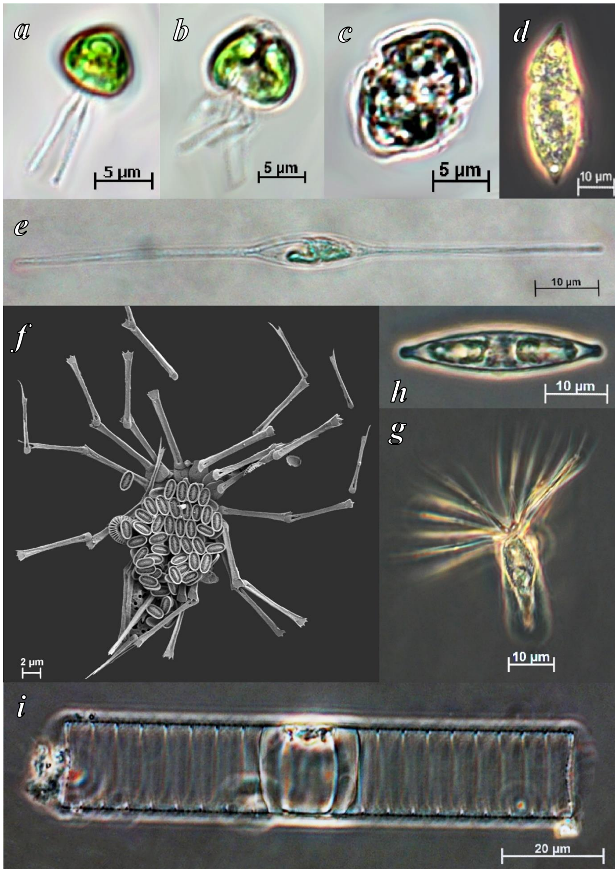
Fig. 15. Micrographs of dominant taxa found at ST1: a) & b) Phytoflagellates; c) Gymnodinium sp.; d) Gyrodinium sp.; e) Nitzschia longissima ; f) & g) Michaelisarsia adriaticus ; h) Nitzschia braarudii ; i) Leptocyliodrus mediterraneus .
