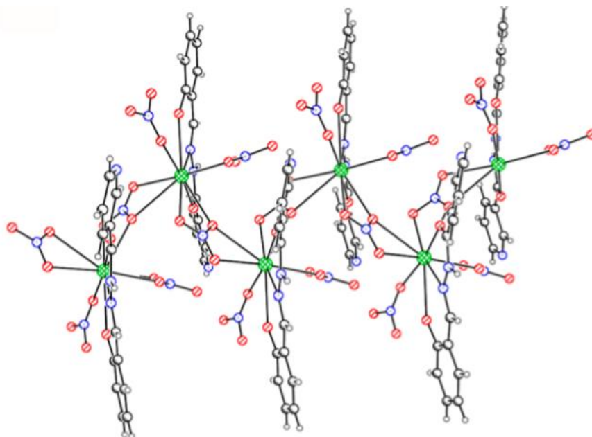
Slika 23. Prikaz 1D zig-zag lanca kompleksa [\text{Pb}(\text{C}_{13}\text{H}_{10}\text{N}_6\text{O}_{11})]_n
