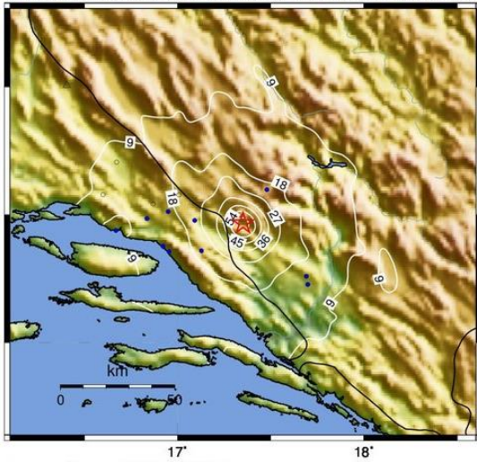
INGV 0.3 s PSA (%g) : Posusje, Bosnia and Herzegovina 21 Jun 2009 11:20:02 UTC M 4.8 N43.47 E17.35 Depth: 2.8km ID:200906211120
