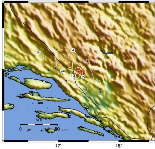
INGV 1.0 s PSA (%g) : Posusje, Bosnia and Herzegovina 21 Jun 2009 11:20:02 UTC M 4.8 N43.47 E17.35 Depth: 2.8km ID:200906211120
