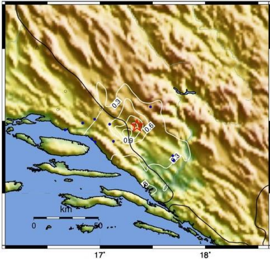
INGV 3.0 s PSA (%g) : Posusje, Bosnia and Herzegovina 21 Jun 2009 11:20:02 UTC M 4.8 N43.47 E17.35 Depth: 2.8km ID:200906211120
