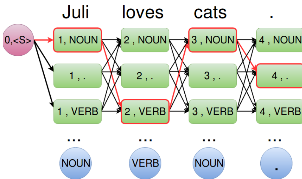
Figure 3.3: Graphical representation of Viterbi algorithm for POS tagging. If the input in Viterbi algorithm is a sentence Juli loves cats. then the output should be NOUN VERB NOUN . . Arrows represent transitions between states and as such they have weights equal to transition probabilities.
