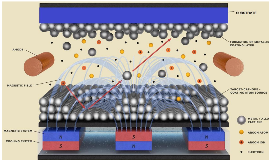
Figure 7. Magnetron sputtering scheme. The static magnetic field is used to contain the plasma near the surface and enhance the sputtering efficiency.
