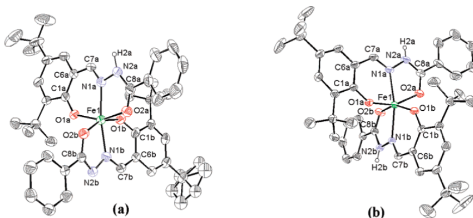
Slika 2.25. ORTEP strukture: a) [\text{Fe}(\text{L-H})(\text{L-2H})] i b) kompleksnog kationa [\text{Fe}(\text{L-H})_2]^+ . 53
