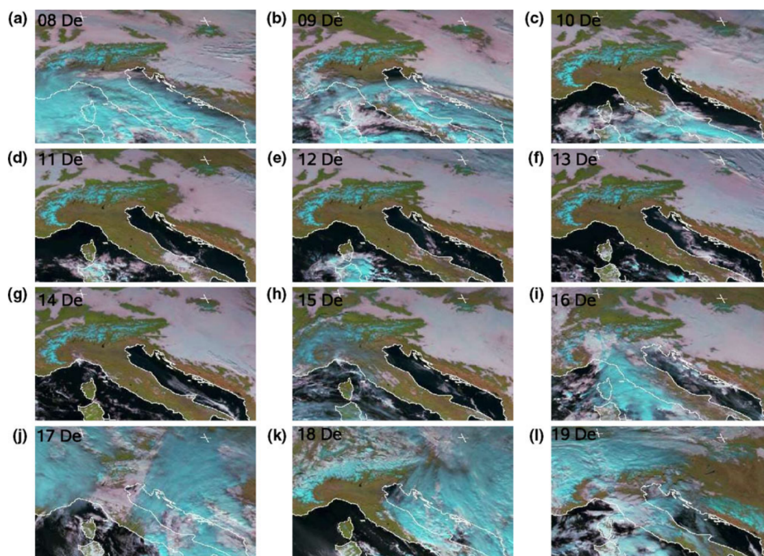
Figure 5.2: Fig. 1 Meteosat-8 satellite images for the period 819 of December 2004, 12 UTC (the dates are written in the panels) composites of channels 1 ( 0.560.71 \mu\text{m} visible), 2 ( 0.740.88 \mu\text{m} visible) and 3 ( 1.501.78 \mu\text{m} near-infrared). Cold ice clouds and snow are in light bluegreen colour, water droplet clouds in pink, the ground in brown and the sea and lake surfaces in black.
