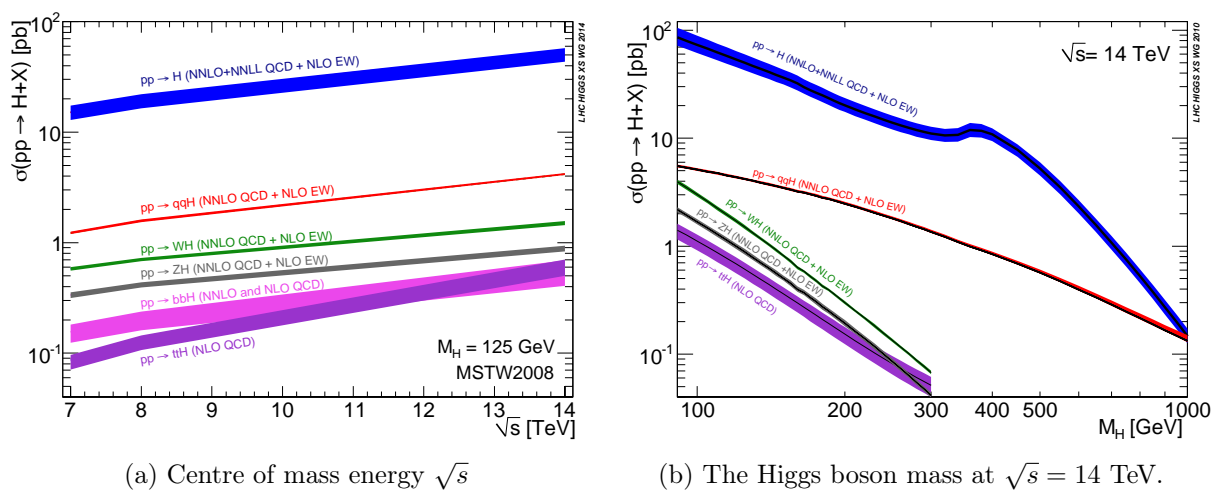
Figure 2.4: The Higgs boson production cross section as a function of the LHC centre of mass energy and its mass at \sqrt{s} = 14 \text{ TeV} .
