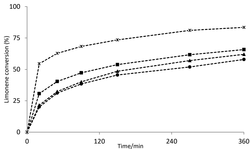
Figure 25. Converted limonene vs. time with polynuclear dioxomolybdenum(VI) complexes and POM hybrid complex: \blacktriangle [\text{MoO}_2(5\text{MeO-SalTSC-4-Ph})]_n , \blacksquare [\text{MoO}_2(5\text{MeO-SalTSC-4-Me})]_n , \bullet [\text{MoO}_2(5\text{MeO-SalTSC})]_n and * [\text{MoO}_2(\text{H5MeO-SalTSC-4-Me})(\text{CH}_3\text{CN})]_2\text{Mo}_6\text{O}_{19} . Reaction conditions: catalyst/limonene/TBHP molar ratio: 0.05/100/200, T = 353 \text{ K} .
