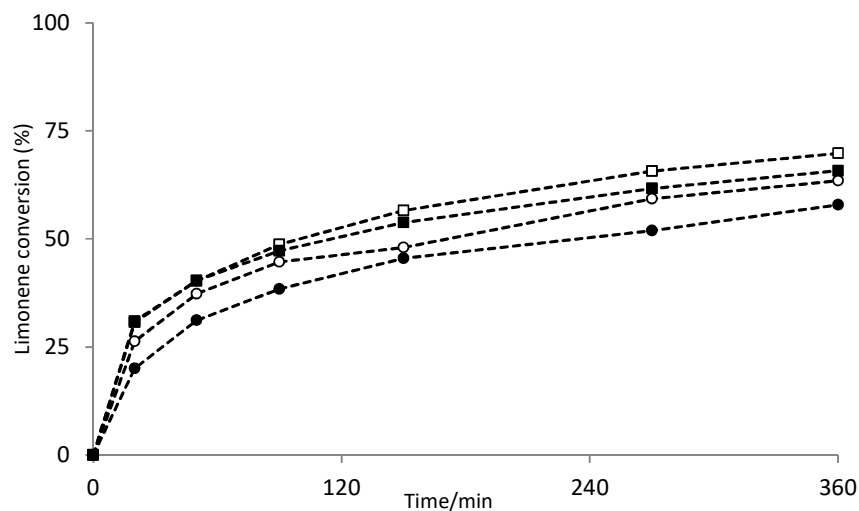
Figure 26. Converted limonene vs. time with polynuclear and mononuclear dioxomolybdenum(VI) complexes: \blacksquare [\text{MoO}_2(5\text{MeO-SalTSC-4-Me})]_n , \bullet [\text{MoO}_2(5\text{MeO-SalTSC})]_n , \square [\text{MoO}_2(5\text{MeO-SalTSC-4-Me})(\text{MeOH})] , \circ [\text{MoO}_2(5\text{MeO-SalTSC})(\text{MeOH})] . Reaction conditions: catalyst/limonene/TBHP molar ratio: 0.05/100/200, T = 353 \text{ K} .
