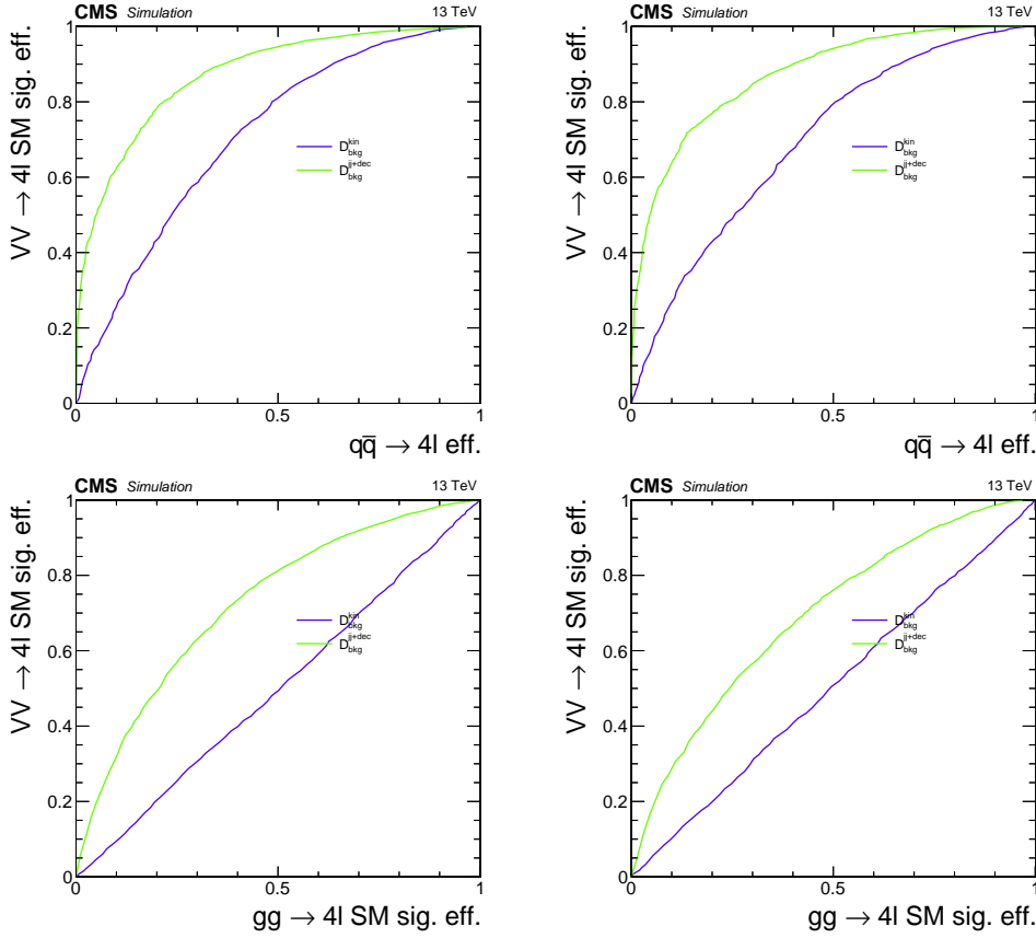
Figure 4.20 – Top left: Comparison of \mathcal{D}_{\text{bkg}}^{\text{VBF}+\text{dec}} and \mathcal{D}_{\text{bkg}}^{\text{kin}} in the VBF-2jet tagged category in terms of efficiency for the VBF signal and q\bar{q} \rightarrow ZZ background. Top right: Comparison of \mathcal{D}_{\text{bkg}}^{\text{VH}+\text{dec}} and \mathcal{D}_{\text{bkg}}^{\text{kin}} in the VH-hadronic tagged category in terms of efficiency for the VH signal and q\bar{q} \rightarrow ZZ background. Bottom left: Comparison of \mathcal{D}_{\text{bkg}}^{\text{VBF}+\text{dec}} and \mathcal{D}_{\text{bkg}}^{\text{kin}} in the VBF-2jet tagged category in terms of efficiency for the VBF and ggH. Top right: Comparison of \mathcal{D}_{\text{bkg}}^{\text{VH}+\text{dec}} and \mathcal{D}_{\text{bkg}}^{\text{kin}} in the VH-hadronic tagged category in terms of efficiency for the VH and ggH. Events are required to pass the full analysis selection and to be in a 105 < m_{4\ell} < 140 GeV window.
