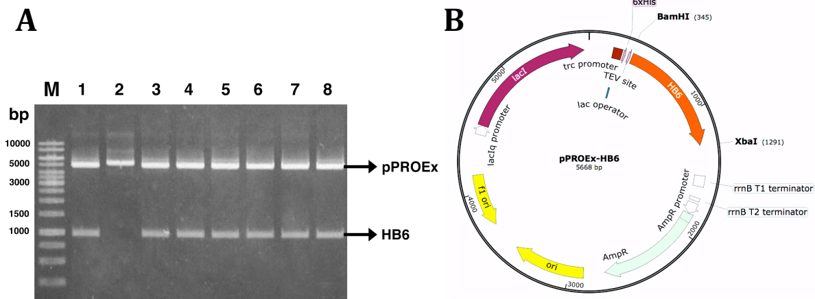
Figure 7. Restriction verification of pPROEx-HB6 construct (A) and its plasmid map obtained in SnapGene program (B) . Recombinant pPROEx-HB6 was digested with BamHI and XbaI. Only two observed bands indicated complete digestion. Expected bands of HB6 insert (946 bp) and pPROEx vector (4722 bp) became visible (depicted with an arrow). M is GeneRuler 1 kb DNA Ladder (Thermo Scientific). Individual minipreps are numbered 1-8. Colony in lane 2 most likely contains an unrestricted plasmid vector.
