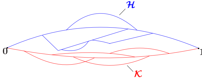
Figure 1.20: \mathcal{H} and \mathcal{K} are TLG*'s.
