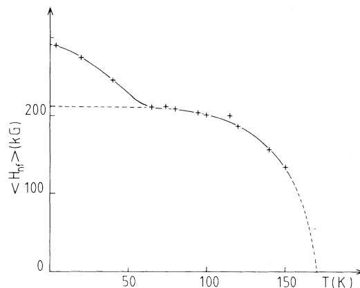
FIG. 2. Average hyperfine field as a function of temperature.
