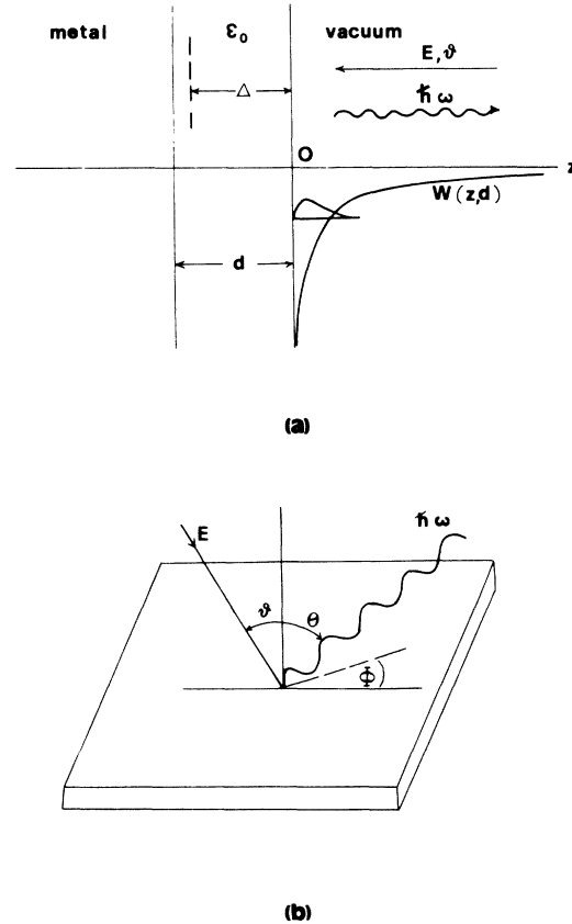
FIG. 1. (a) Energy scheme for electrons trapped in the image potential W(z, d) on a layer of dielectric ( -d < z < 0 ) deposited on a metal substrate ( z < -d ). |R|^2 is the reflectivity of incoming electrons at the surface, \delta is the scattering phase shift, and \Delta defines the reflection plane of impinging electrons. (b) Geometry of the system, with incoming electron ( \vartheta ) and emitted photon angles ( \theta, \Phi ).
