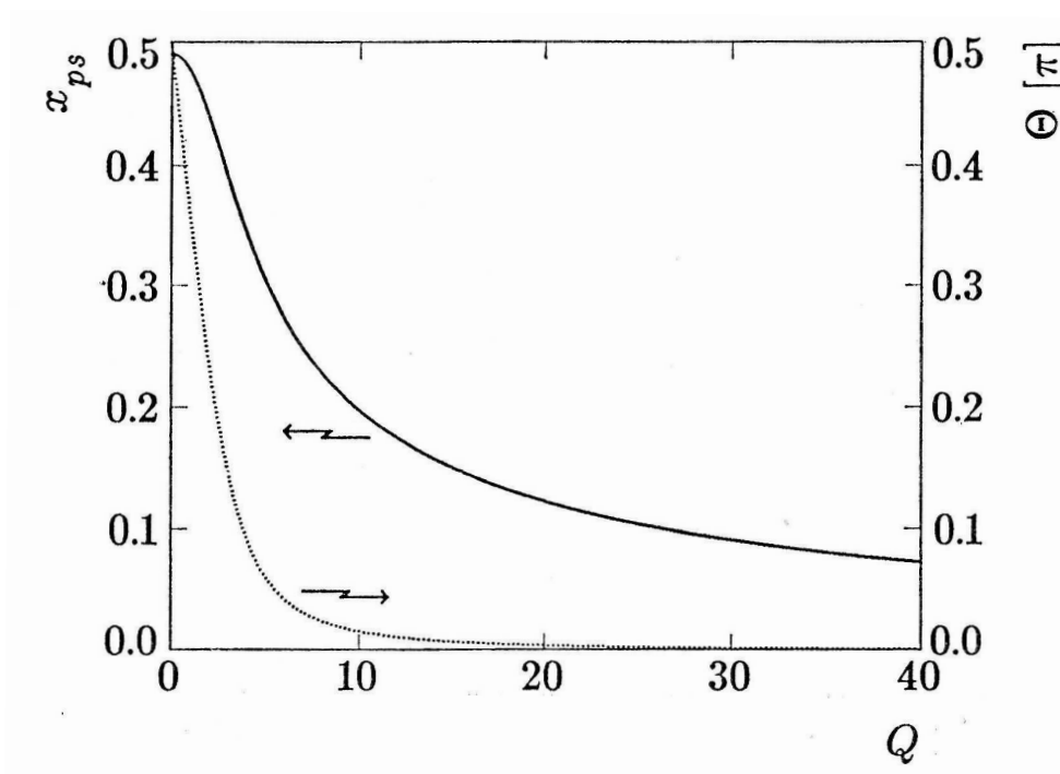
Fig. 2. (a, previous page) The dependence of \alpha and \beta , Eq. (20) on Q for E = 10 . For Q = 0 , \alpha = \beta = \sqrt{E/2} . (b) The corresponding distance x_{ps} (Eq. (21a)) of the PS-plane from the boundary for |\Delta_0| = 1 , and the angle \theta (Eq. (29)) of the equiphase lines \Phi(x \rightarrow 0) = \Phi_0 with respect to the x -axes.
