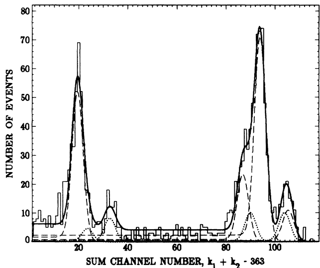
FIG. 2. The histogram shows the sum spectrum made from the data in a central region of the E_1 - E_2 two-dimensional spectrum of the hafnium experiment, for x = E/E_0 in a range between about 0.35 to about 0.65. The dashed curves show (in the order from the left to the right) the peaks of the fitting functions due to the 2s \rightarrow 1s , 3s \rightarrow 1s , 3d \rightarrow 1s , and 4sd \rightarrow 1s two-photon decay. The dotted curves show (again in the order from the left to the right) the fitting functions due to the crosstalk via backscattered Compton radiation from the K\alpha_2 , K\alpha_1 , K\beta_1 , and K\beta_2 x rays of hafnium. The heavy solid line shows the sum of the above fitting functions and of a constant background.
