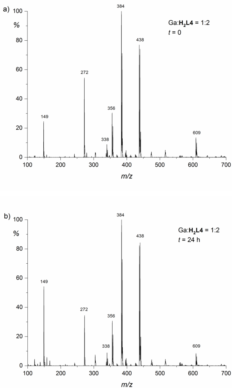
Slika D3. Spektri masa otopine galijeve(III) perklorata i hidrazona \text{H}_2\text{L}_4 u omjeru 1:2 ( c(\text{H}_2\text{L}_2) = 5 \times 10^{-4} \text{ mol L}^{-1} , c(\text{Ga}^{3+}) = 2,5 \times 10^{-4} \text{ mol L}^{-1} ) u otapalu metanol/voda 1/1 uz perklornu kiselinu ( c(\text{HClO}_4) = 0,003 \text{ mol L}^{-1} ; \text{pH} = 2,52 ) odmah po pripravi otopine (a) i nakon 24 sata (b)
