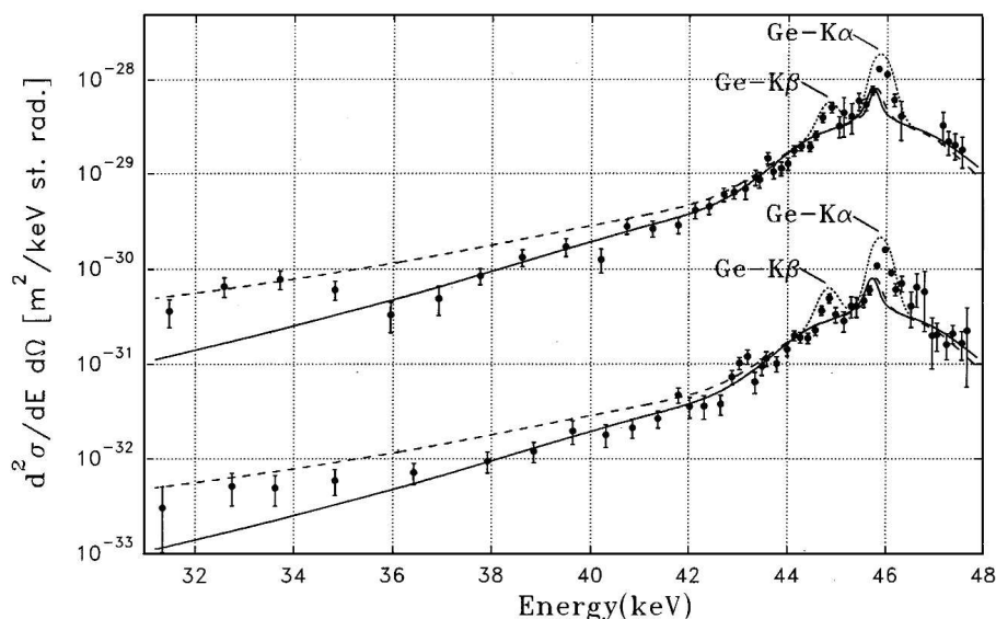
Fig. 2. Compton profile for incident photons of 55.791 keV. Experimental data are shown by full circles. Full line and dashed lines show the results of calculations using the impulse and the "A 2 -Born" approximation, respectively, and the dotted lines shows the sum of the results of calculations for the cross-talk between the detectors via Ge K X-rays and of the impulse approximation. Upper data are due to the detector 1 and lower data (multiplied by the factor 0.01) are due to the detector 2.
