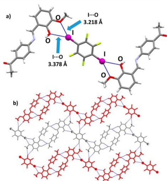
Figure 5. Form B of (\text{ov4aa})_2(\text{14tfib}) : (a) molecular complex formed by \text{I}\cdots\text{O} halogen bonds and (b) chains (red and gray) connected into a sheet via hydrogen bonds.
