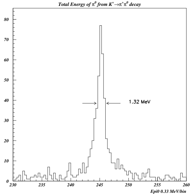
Fig. 2. A spectrum of \pi^0 from the decay, K^+ \rightarrow \pi^0\pi^+ , showing the NMS resolution.
