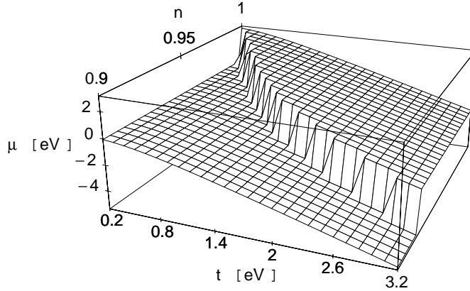
Fig. 1. The chemical potential \mu of the mobile spins, as a function of the hopping overlap t and doping n = 2n_{\uparrow} = 2n_{\downarrow} . Electron doping is n < 1 , and \Delta_{pd} = 3 eV, T = 40 K throughout.
