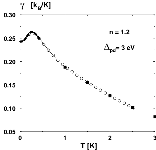
Fig. 2. Scaling property of the linear specific heat coefficient, for n = 1.2 and various t . Squares: t = 0.2 eV. Circles: t = 0.3 eV, range to 12 K scaled by c = 4.75 in Eq. (5). Full line: t = 0.8 eV, range to 100 K, c = 127.4 . Dashed line: t = 1.0 eV, range to 100 K, c = 232.7 .
