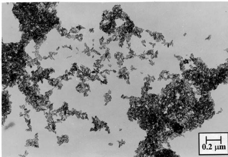
Figure 15. Transmission electron micrograph of sample S62.
