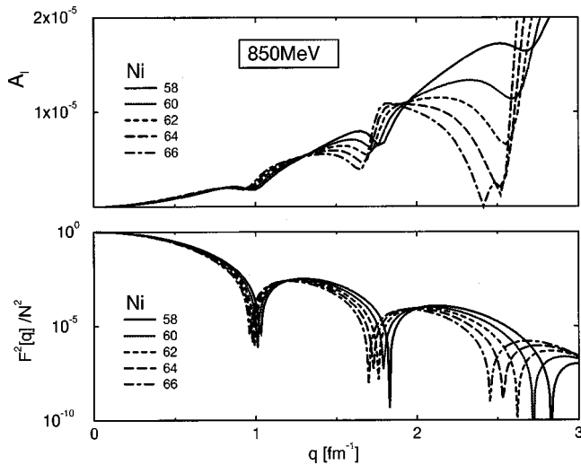
FIG. 10. Parity-violating asymmetry parameters A_l (upper panel) and squares of normalized Fourier transforms of neutron densities (lower panel), as functions of the momentum transfer q , for elastic scattering from ^{58-66}\text{Ni} at 850 MeV.
