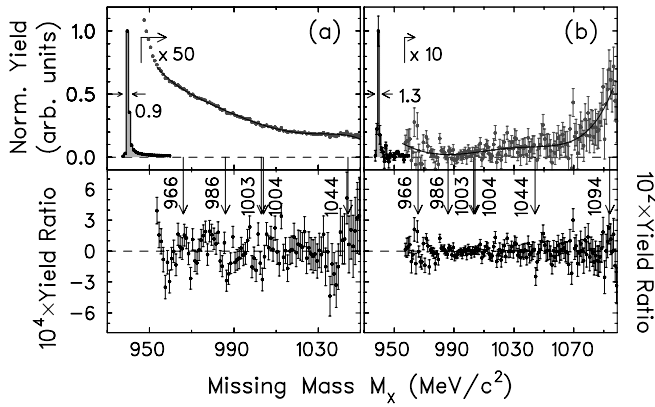
FIG. 4. Upper half: Missing-mass spectra of the {}^2\text{H}(e, e'p)X reaction in the region near the quasielastic peak at (a) Q^2=0.6 to 0.7 ( \text{GeV}/c^2 ) and (b) Q^2=0.8 to 1.1 ( \text{GeV}/c^2 ) (with the neutron peak height set to unity). The plot shows the combined settings (a) D-4,5 and (b) D-8,9,10 (with the spectrometer settings listed in Table II). The achieved missing-mass resolution is (a) \approx 0.9 \text{MeV}/c^2 and (b) \approx 1.3 \text{MeV}/c^2 . The solid curves and the yield ratios in the lower half are obtained in the same way as in Fig. 1. Significant structures are excluded to a level of (a) 10^{-4} and (b) 10^{-2} of the height of the neutron peak, respectively.
