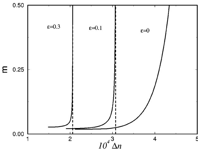
FIG. 2. The modulation depth vs \Delta n = \gamma I^{(0)} for different values of \epsilon ; \theta = 0.0096 , and I_S = \infty . m is shown from the instability threshold up to the cavity threshold (indicated by vertical dashed lines).
