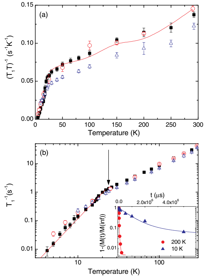
FIG. 4 (color online). (a) The ^{75}\text{As} (T_1T)^{-1} versus temperature in \text{LaFeAsO}_{0.9}\text{F}_{0.1} measured at the upper horn ( \blacksquare ) ( \theta = 90^\circ ), the lower horn (blue \triangle ) ( \theta \approx 41.8^\circ ), and in the aligned sample (red \circ ) ( \theta = 90^\circ ). The solid line is given by K_s^2(T)/\alpha\kappa as described in the text. (b) T_1^{-1} versus temperature. The arrow indicates T_c = 23.5 K at 7 T, and the solid line indicates T_1^{-1} \sim T^3 , indicative of line nodes. Inset: Magnetization recovery and fits for two temperatures.
