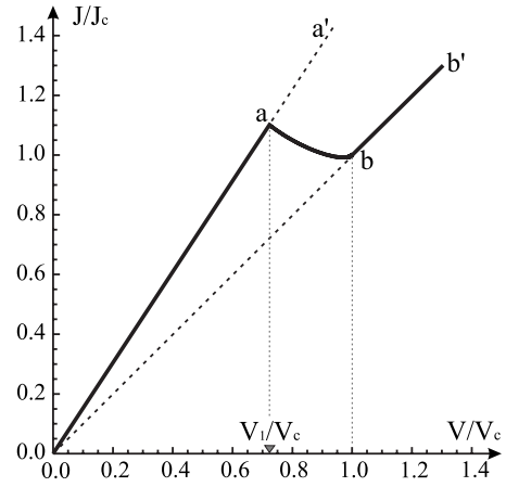
FIG. 5. IVC of the magnetic stack of Fig. 1 calculated for R(\Theta)=R_+ , -R_- \cos \Theta , R_+/R_+=0.2 , and D_0=0.2 ; J_c=V_c/R(\pi) . The branches 0– a and b – b' of the IVC correspond to parallel and antiparallel orientations of the stack magnetization, respectively (the parts a – a' and 0– b are unstable); the branch a – b corresponds to the inhomogeneous magnetization distribution shown in Fig. 2.
