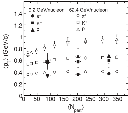
FIG. 12. \langle p_T \rangle for \pi^+ , K^+ , and p plotted as a function of \langle N_{\text{part}} \rangle for Au + Au collisions at \sqrt{s_{NN}} = 9.2 GeV and compared with corresponding results at \sqrt{s_{NN}} = 62.4 GeV [4,23,37]. The errors shown are the quadrature sum of statistical and systematic uncertainties. The systematic errors for pions, kaons, and protons for \sqrt{s_{NN}} = 9.2 GeV are \sim 12\% , 18\% , and 21\% , respectively, and similar for all the collision centralities studied.
