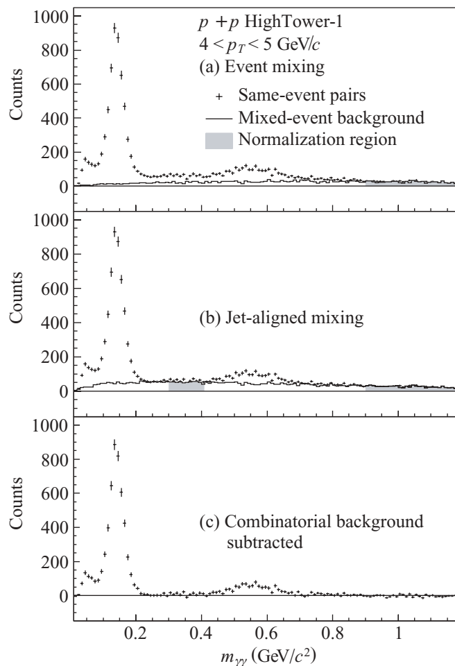
FIG. 7. The same-event invariant mass distribution (crosses) and combinatorial background (histogram) observed in one p_T bin of the p+p data. Background estimated (a) from random event mixing and (b) from a linear combination of random and jet-aligned mixing; (c) background-subtracted distribution. The shaded areas indicate the regions where the mixed-event background was normalized to the same-event distributions.
