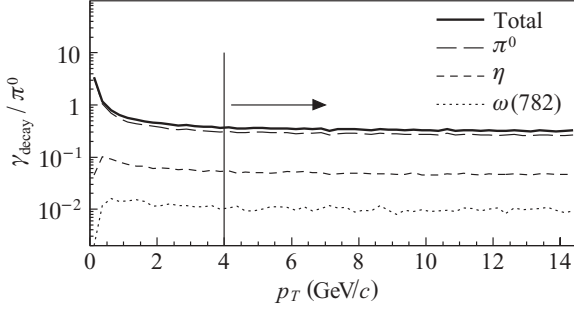
FIG. 21. The simulated number of photons per input pion \gamma_{\text{decay}}/\pi^0 from hadronic decays in d + Au collisions as a function of p_T . The included decay processes are listed in Table IV. The vertical line indicates the lower limit of the p_T range that was used to fit the \pi^0 spectrum. The value of \gamma_{\text{decay}}/\pi^0 below p_T = 4 GeV/c is, therefore, less accurate; however, it was not used for further analysis (see text).
