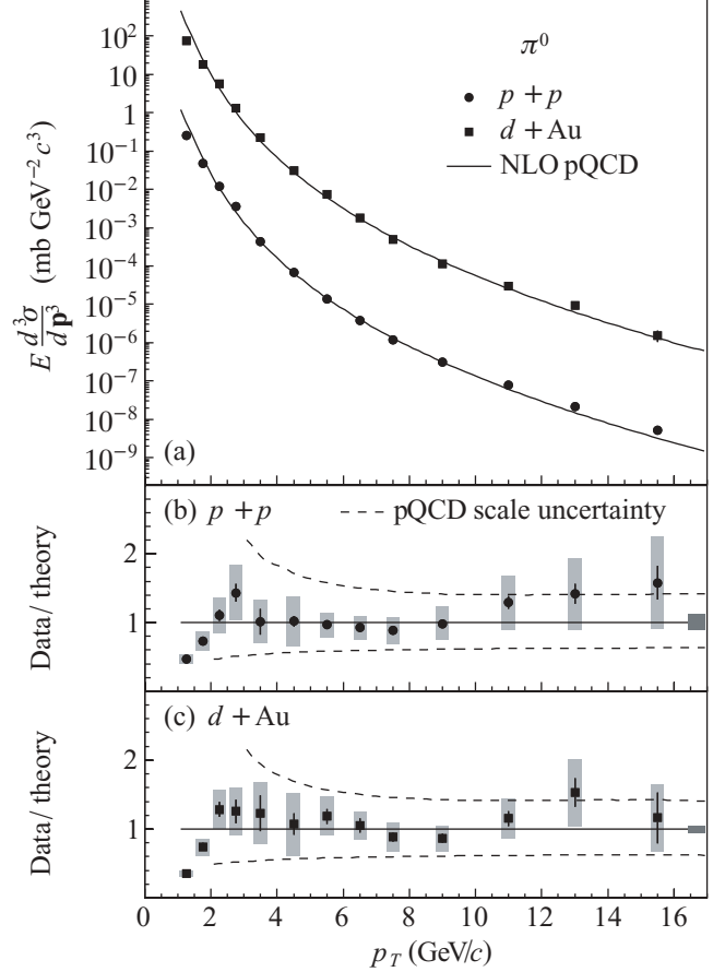
FIG. 22. (a) Cross section for inclusive \pi^0 production in p + p and d + Au collisions at \sqrt{s_{NN}} = 200 GeV, divided by the corresponding NLO pQCD calculations [52] for (b) p + p and (c) d + Au collisions. The error bars are statistical and shaded bands are p_T -correlated systematic uncertainties. Normalization uncertainties are indicated by shaded bands around unity in the lower panels.
