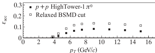
FIG. 14. Acceptance and efficiency correction factor \epsilon_{\text{acc}} for the p + p HighTower-1 data, with the standard set of cuts (solid symbols) and with the SMD quality cut removed (open symbols).
