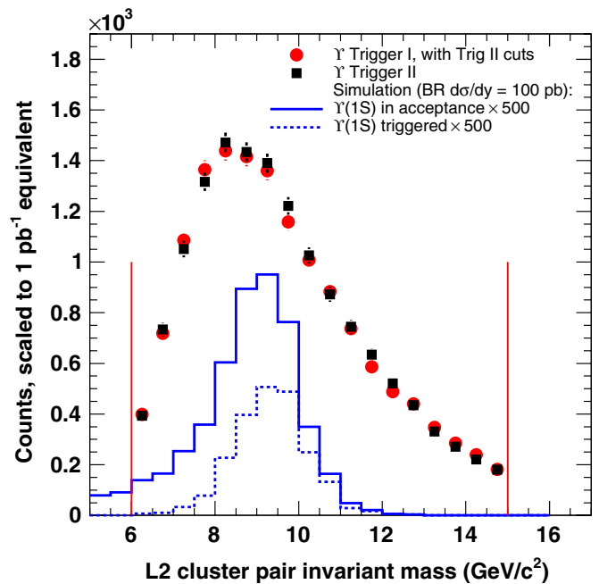
FIG. 6 (color online). The L2 invariant-mass M_{12}^{L2} distribution for accepted events. The line histograms show the \Upsilon M_{12}^{L2} distribution after acceptance requirements (solid line), and after all trigger requirements (L0 HTTP trigger, L2 cluster, L2 opening angle, and L2 invariant mass) of the e^+e^- daughters (dashed line). Vertical lines show location of the trigger thresholds. Normalization and scaling factors are the same as in Fig. 3.
