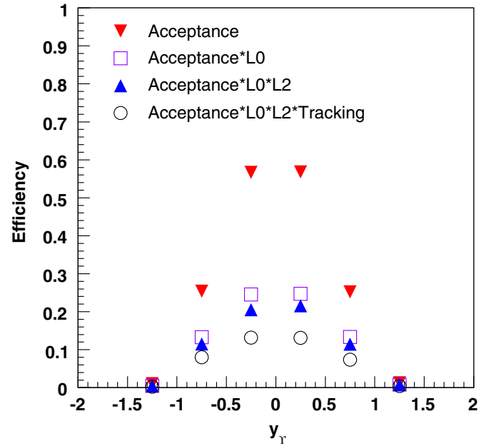
FIG. 7 (color online). Combined acceptance \times efficiency as a function of rapidity y_Y for the decay Y \rightarrow e^+e^- in STAR. Downward triangles: BEMC acceptance only; open squares: adding L0 requirement; upright triangles: adding L2 requirement; open circles: adding TPC acceptance + TPC tracking cuts and TPC-BEMC matching.
