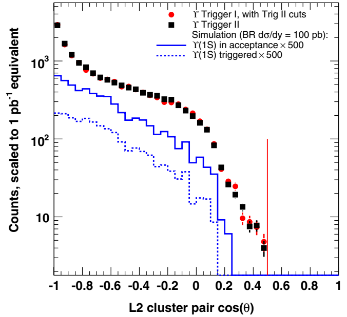
FIG. 5 (color online). The distribution of cosine of L2 opening angle \theta_{12}^{L2} for accepted events. The line histograms show the \Upsilon distribution after acceptance requirements (solid line), and after all trigger requirements (dashed line). The vertical line shows the location of the trigger threshold. Normalization and scaling factors are the same as in Fig. 3.
