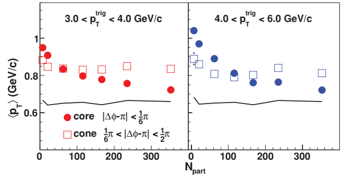
FIG. 9. (Color online) Mean transverse momentum \langle p_T \rangle(\Delta\phi) of associated hadrons in the range 0.25 < p_T^{\text{assoc}} < 4.0 GeV/c in the core ( |\Delta\phi - \pi| < \frac{\pi}{6} ) and cone ( \frac{\pi}{6} < |\Delta\phi - \pi| < \frac{\pi}{2} ) azimuthal regions for 3 < p_T^{\text{trig}} < 4 and 4 < p_T^{\text{trig}} < 6 GeV/c as a function of number of participants. The lines indicate the inclusive \langle p_T \rangle in the same p_T range for events with a trigger hadron.
