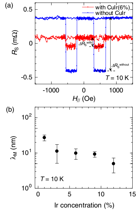
FIG. 2 (color online). (a) NLSV signals measured at T = 10 \text{ K} with a CuIr (6%) middle wire (red) and without CuIr wire (blue). (b) Spin diffusion length \lambda_{\text{M}} of CuIr at 10 \text{ K} as a function of Ir concentration.
