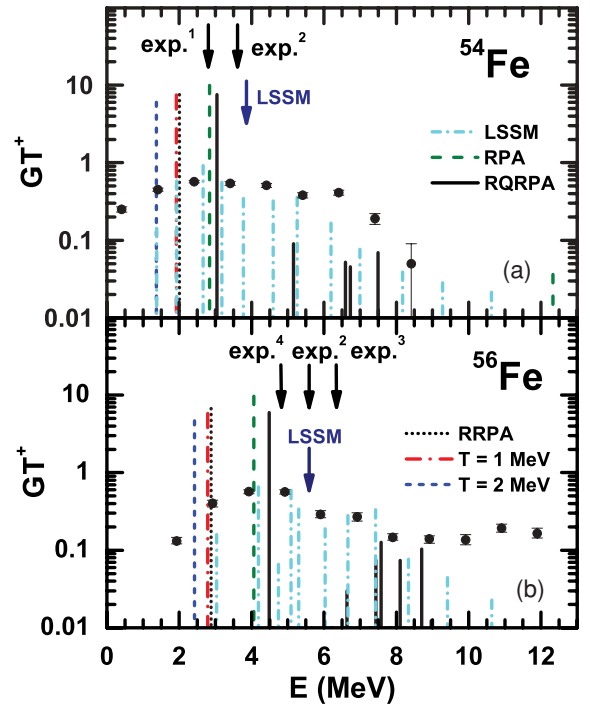
FIG. 1. (Color online) The \text{GT}^+ strength distributions for ^{54,56}\text{Fe} as functions of the excitation energy with respect to the ground state of the parent nucleus, calculated with the proton-neutron RQRPA at zero temperature, and the FTRRPA at T = 0, 1, and 2 MeV, for the DD-ME2 relativistic density functional. For comparison, the \text{GT}^+ strength calculated with the nonrelativistic RPA based on the SLy5 Skyrme functional (green dashed lines), and the centroid energies (blue arrows) and distributions of the LSSM calculation [11] at T = 0 MeV are shown. The experimental centroid energies from Refs. [47–50] are indicated by black arrows, and the experimental distributions from Ref. [48] for ^{54}\text{Fe} and Ref. [49] for ^{56}\text{Fe} are shown by solid circles.
