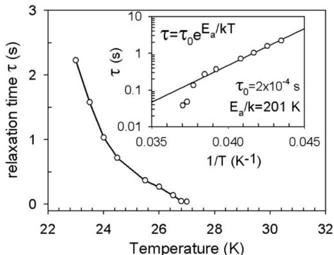
FIG. 3. Temperature dependence of the mean relaxation time (main panel) obeys the Arrhenius-type thermal activation with approximately temperature-independent activation energy E_a (inset). E_a is unusually big due to strong magnetocrystalline anisotropy K resulting from the strong single-ion anisotropy energy.
