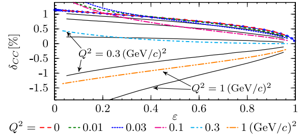
FIG. 1 (color online). Comparison of Coulomb corrections.
