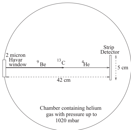
FIG. 1. Experimental setup showing the ^9\text{Be} beam passing through the Havar window, interacting with a ^{13}\text{C} nucleus to form ^{13}\text{C} , with the subsequent emission of an \alpha particle in the forward direction. The \alpha particle is then detected by the silicon strip detector. The gas pressure is then adjusted to stop the beam in the gas before the detector.
