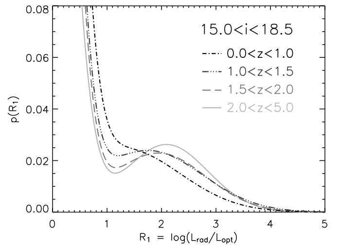
Figure 8. Radio loudness distribution as a function of redshift for flux-limited subsamples of quasars with i < 18.5 . Note that bimodality seems to have been more prominent at high redshift and that it flattened out at low redshift. The same general trend is detectable in fainter subsamples, but the shape of the distribution does not change in a monotonous manner.
