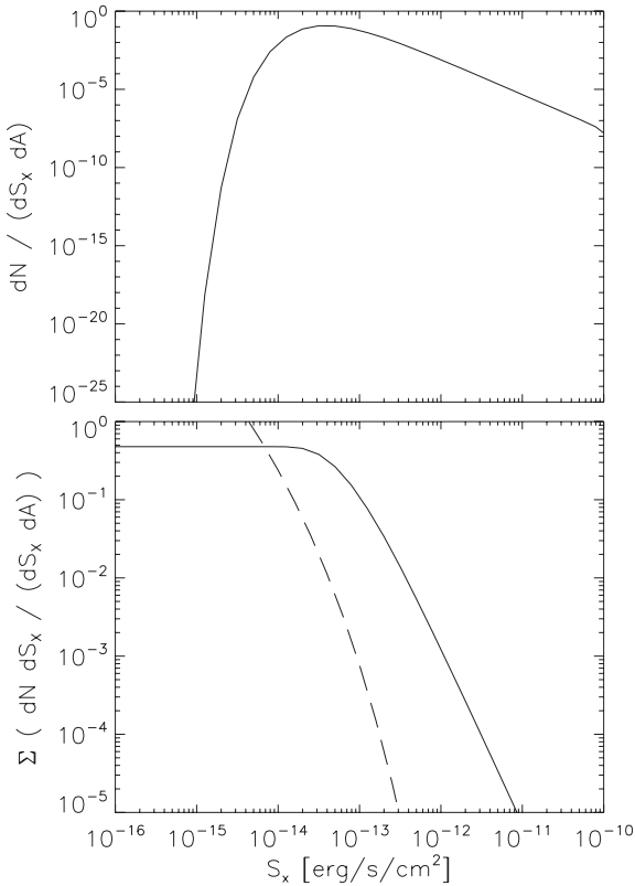
Figure 10. Differential (top panel) and cumulative (bottom panel) number counts (per deg 2 ) as a function of X-ray flux expected for extended IC X-ray sources (solid lines) and for clusters (dashed line). The radio counts were obtained by evolving the radio LF for powerful (FR II) radio galaxies (Willott et al. 2001, covering the range of 10^{25} – 10^{30} W Hz -1 ; see text for details), while the cluster counts, in the redshift range of 1 < z < 3 , were obtained following Finoguenov et al. (2010).
