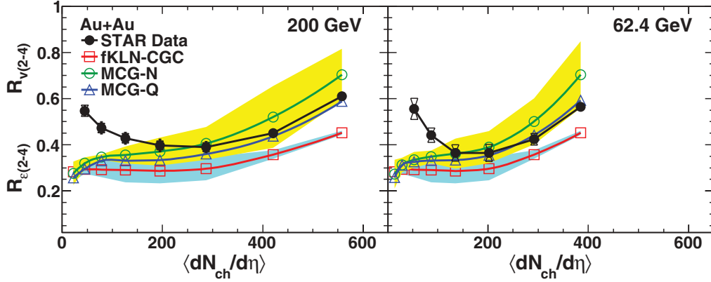
FIG. 6. (Color online) The upper limit on \sigma_{v_2}/\langle v_2 \rangle for 200 GeV (left) and 62.4 GeV (right) Au + Au collisions from Eq. (9) compared to \sigma_\epsilon/\epsilon from Eq. (10) for three different models. The upper limit is found using the LS results for v_2\{2\} . Data are from the range 0.15 < p_T < 2.0 GeV/c. The shaded bands reflect the uncertainties on the models which are dominated by uncertainty on the distribution of nucleons inside the nucleus. The uncertainty is only shown for the MCG-N and fKLN-CGC models. The uncertainty on the MCG-Q model is the same as for the MCG-N model but is not shown for the visual clarity.
