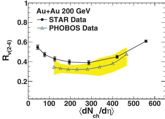
FIG. 7. (Color online) The STAR data compared to PHOBOS data [34] on \sigma_{v_2}/\langle v_2 \rangle with \delta_2 for \Delta\eta > 2 taken to be zero (see Fig. 6 from Ref. [34]). The shaded band shows the errors quoted from Ref. [34].
