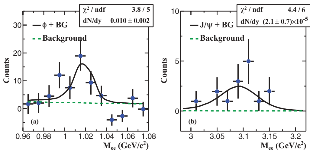
FIG. 16. (Color online) (a) The M_{ee} distribution after the mixed-event background subtraction for 0.96 < M_{ee} < 1.08 GeV/ c^2 in p + p collisions at \sqrt{s} = 200 GeV. The curve represents the fit in the range of 0.98 < M_{ee} < 1.04 GeV/ c^2 . Errors on data points are statistical. (b) The M_{ee} distribution after the mixed-event background subtraction for 2.98 < M_{ee} < 3.22 GeV/ c^2 in p + p collisions at \sqrt{s} = 200 GeV. The curve represents the fit in the range of 3 < M_{ee} < 3.16 GeV/ c^2 . There is no count in the unlike-sign and like-sign electron-pair distributions for 3.02 < M_{ee} < 3.04 GeV/ c^2 due to statistical fluctuations. Errors on data points are statistical.
