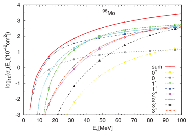
FIG. 5. (Color online) The same as in Fig. 1, but for the scattering process ^{98}\text{Mo}(\nu_e, \nu'_e)^{98}\text{Mo}^* .
