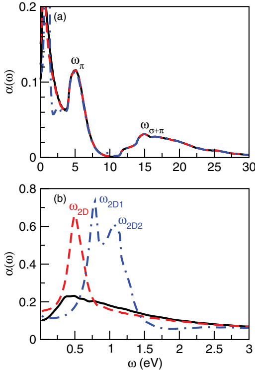
FIG. 3. (Color online) Nonlocal singularity index \alpha(\omega) vs plasmon energy \omega in eV for graphene with dopings of \epsilon_F = 0 (black solid line), \epsilon_F = 0.5 eV (red dashed line), and \epsilon_F = 1 eV (blue dash-dotted line). (a) Broad peaks corresponding to the \pi and \sigma + \pi plasmons. (b) Sharp peaks (with positions increasing with doping) corresponding to 2D or Drude plasmons.
