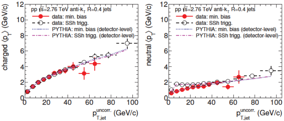
Fig. 76. Mean transverse momentum, \langle p_T \rangle , of constituents measured in reconstructed jets in 2.76 TeV pp collisions (anti- k_T , R = 0.4 ), versus jet p_T . Left: charged tracks; Right: neutral clusters. Data are shown for MB and SSh triggers, and are compared to detector-level simulations.
