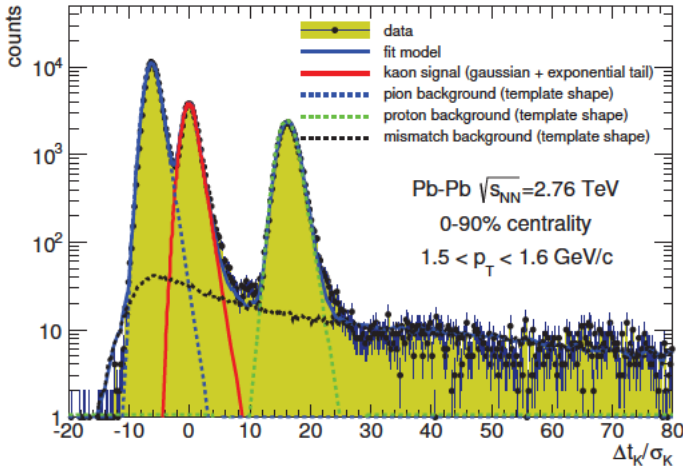
Fig. 42. TOF measured in Pb-Pb collisions at \sqrt{s_{\text{NN}}} = 2.76 TeV. The expected time of flight for kaons is subtracted and the result is divided by the expected resolution.
