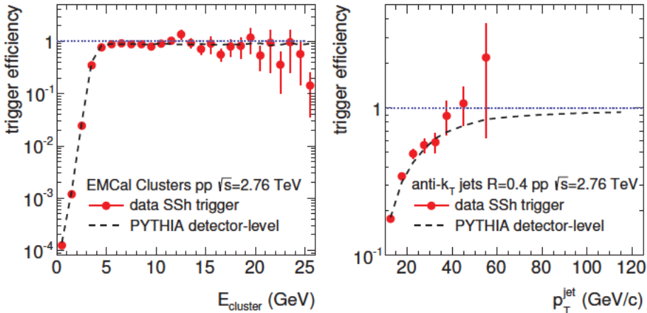
Fig. 73. (Color online) SSh trigger efficiency in pp collisions at \sqrt{s} = 2.76 TeV. Efficiency for single EM clusters (left panel) and reconstructed jets (anti- k_T , R = 0.4 , right panel) for data (red points) is well reproduced in simulation (black dashed line). See text for details.
