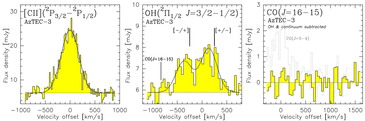
Figure 9. ALMA spectra of the [\text{C II}]({}^2P_{3/2} \rightarrow {}^2P_{1/2}) (left), \text{OH}({}^2\Pi_{1/2} J = 3/2 \rightarrow 1/2) (middle), and \text{CO}(J = 16 \rightarrow 15) (right) lines toward AzTEC-3. Spectra (histograms) are shown at resolutions of 20 MHz ( 20 \text{ km s}^{-1} ; [\text{C II}] ) or 40 MHz ( 41 \text{ km s}^{-1} ; OH and CO). The velocity scales are relative to z = 5.2988 . Detected lines are shown along with Gaussian fits to the line emission (black curves). In the case of OH, zero velocity corresponds to the central frequency between the P components of the \Lambda doublet. The [+/-] and [-/+] labels at \pm 249 \text{ km s}^{-1} indicate the P components of the \Lambda doublet (i.e., J^P = 3/2^+ \rightarrow 1/2^- and 3/2^- \rightarrow 1/2^+ , respectively). Due to the narrow splitting ( \sim 14 and 2 \text{ MHz} observed-frame, respectively), labels for hyperfine structure splitting of the P components are omitted for clarity. OH and continuum emission as quantified by the Gaussian fit in the middle panel have been subtracted from the \text{CO}(J = 16 \rightarrow 15) spectrum. The dashed gray histogram shows the \text{CO}(J = 5 \rightarrow 4) emission (R10) for comparison, which demonstrates that the bulk of the \text{CO}(J = 16 \rightarrow 15) line is covered by the 1.875 GHz bandpass shown.
