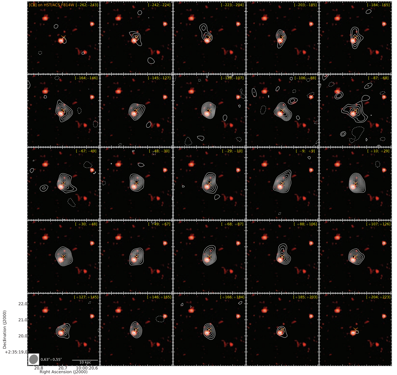
Figure 5. ALMA [\text{C II}]^2P_{3/2} \rightarrow ^2P_{1/2} velocity channel contours overlaid on the HST/ACS F814W image toward AzTEC-3. Velocity channels are averaged over \sim 19.53 MHz ( \sim 19 km s ^{-1} ). Contours start at \pm 3\sigma and are in steps of 1\sigma ( 1\sigma = 974 \mu\text{Jy beam}^{-1} at the phase center). The noise close to -70 km s ^{-1} is slightly higher due to a weak atmospheric absorption feature (see Section 2). Velocity ranges in km s ^{-1} are indicated in the top right corner of each panel. The synthesized beam size is the same as in Figure 3. The velocity scale is the same as in Figure 3. The crosses and plus signs indicate the same positions as in Figure 3.
