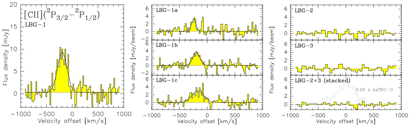
Figure 10. ALMA [\text{C II}]({}^2P_{3/2} \rightarrow {}^2P_{1/2}) spectra toward LBG-1 (left) and its components LBG-1a, LBG-1b, and LBG-1c (middle; see Figure 7), as well as LBG-2 and LBG-3 (right). Spectra (histograms) are shown at resolutions of 19.5 MHz ( 19 \text{ km s}^{-1} ; left and middle) or 39 MHz ( 39 \text{ km s}^{-1} ; right). The left spectrum corresponds to the spatially integrated emission shown as contours in Figure 7. The middle and right spectra are extracted at the optical peak positions for all sources (plus signs in Figures 1 and 7). The velocity scales are relative to z = 5.2988 . Detected lines are shown along with Gaussian fits to the line emission (black curves). The bottom right panel shows a stack of the spectra of LBG-2 and LBG-3. The dashed gray histogram shows the [\text{C II}]({}^2P_{3/2} \rightarrow {}^2P_{1/2}) emission from the strong nearby source AzTEC-3 (Figure 9), scaled by a factor of 0.25, for comparison.
